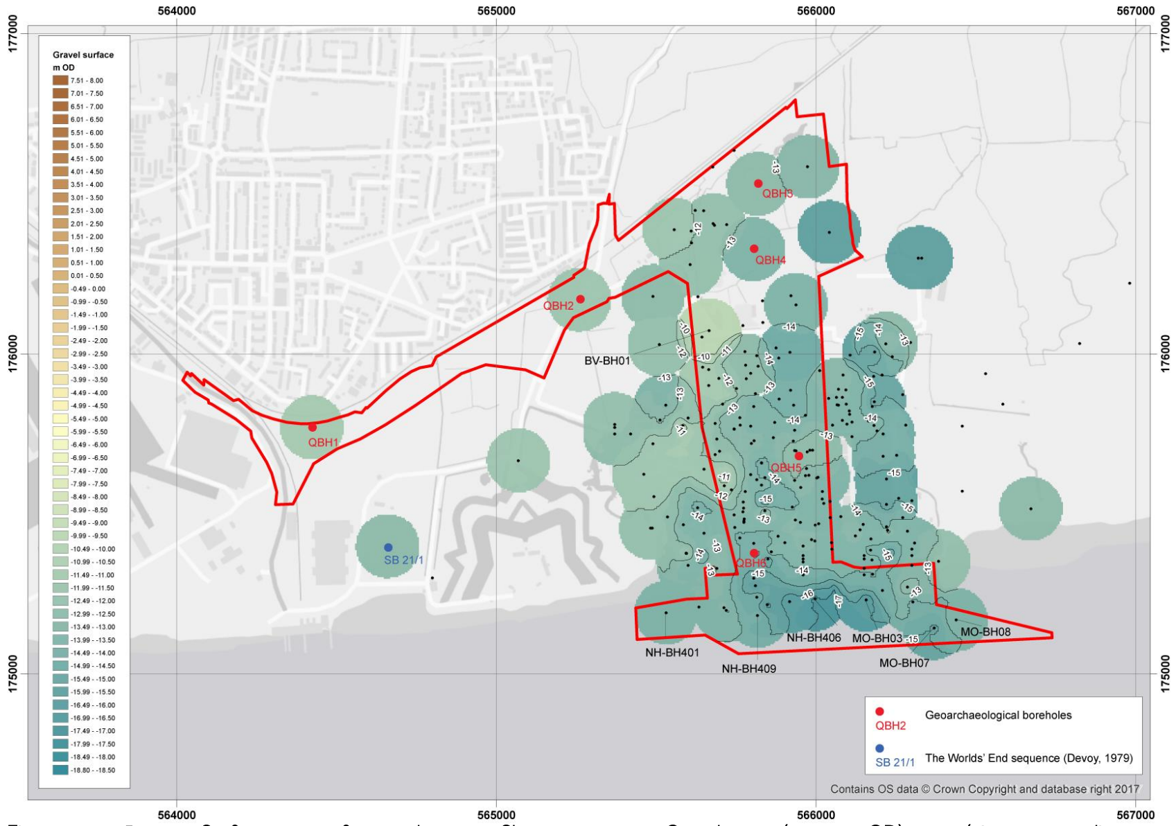
Figure 5: Surface of the Shepperton Gravel (m OD) (site outline in red).
